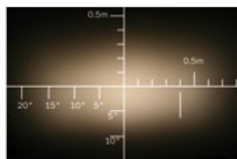
27° Medium Reflector - Glare Control & #555 Glass
