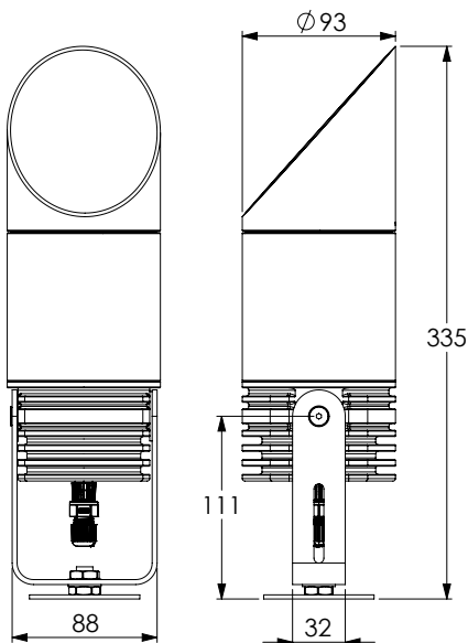
COWL + PLUG IN CABLE OPTION WITH EXTENDED STIRRUP DIMENSIONS
